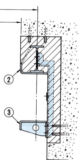
SECTION "Z," UPPER GUIDE 上部戸当
