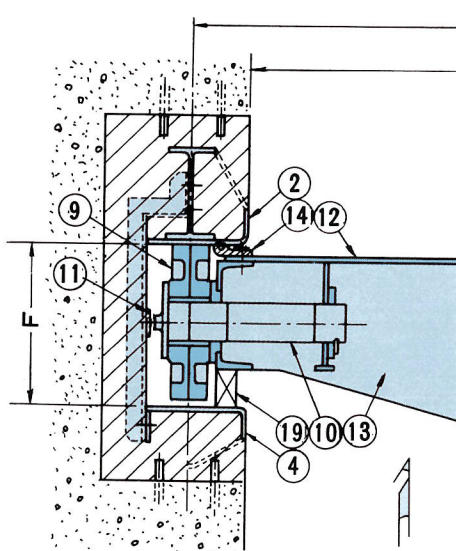
SECTION "U," SIDES WATER TIGHTNESS 側部水密
